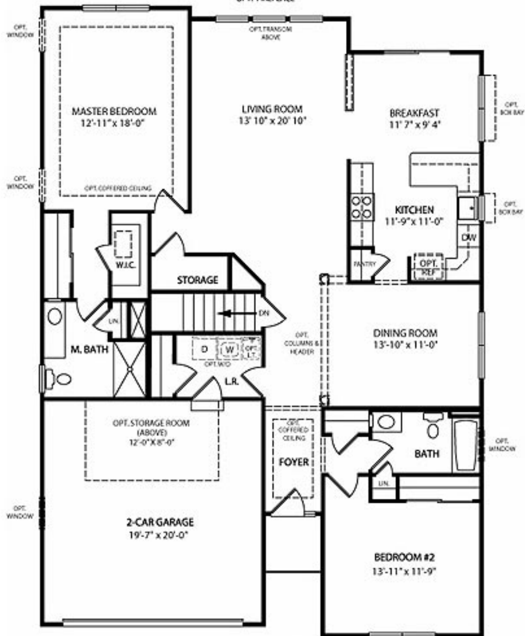
FIRST FLOOR PLAN "B"
