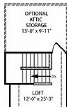
OPT. LOFT W/ OPT. STORAGE PLAN
