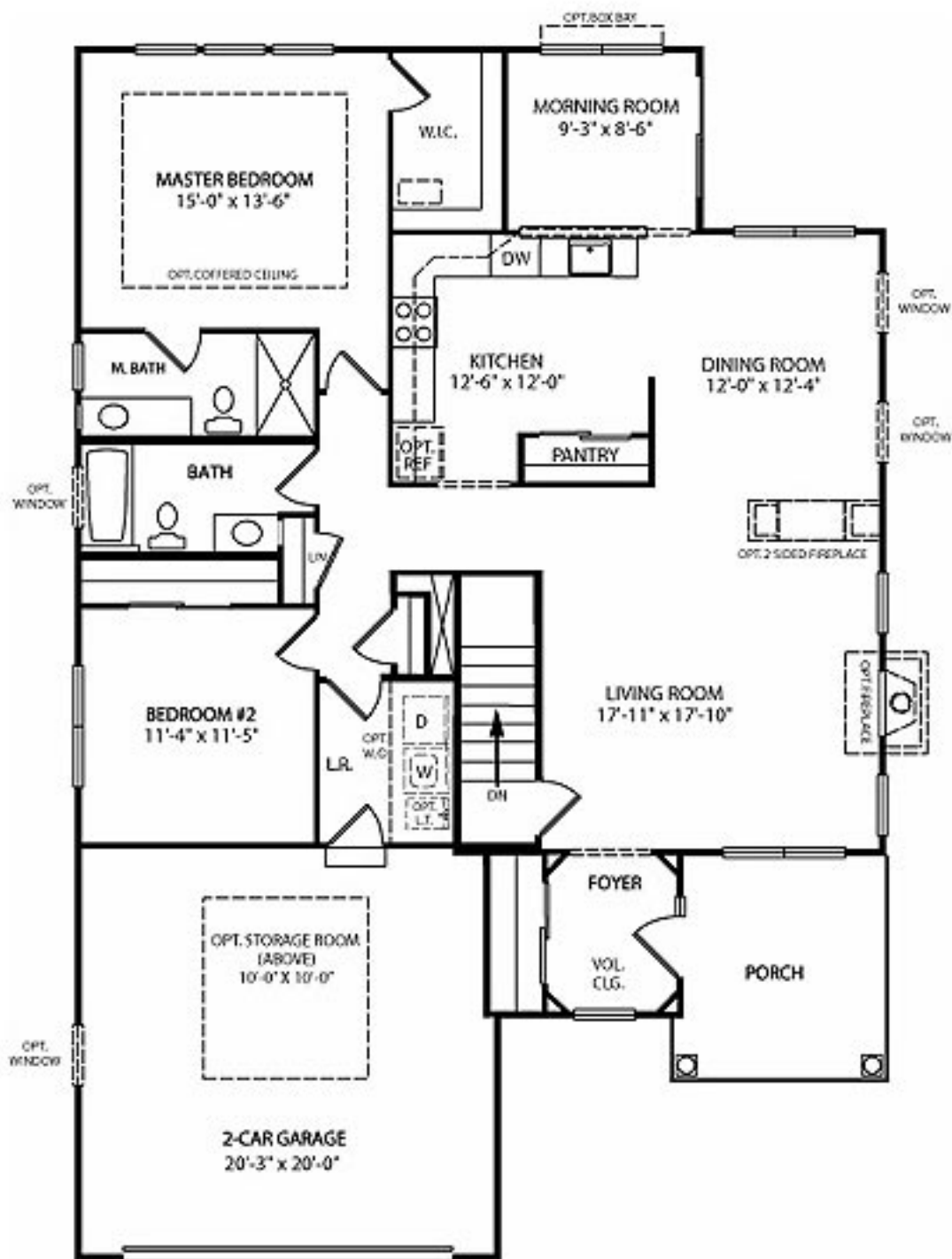
FIRST FLOOR PLAN "A"
