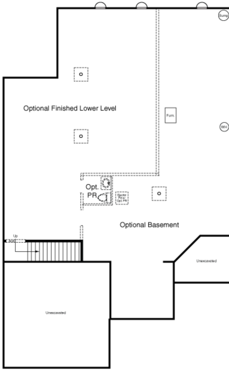
Cordova Finished Basement Plan
