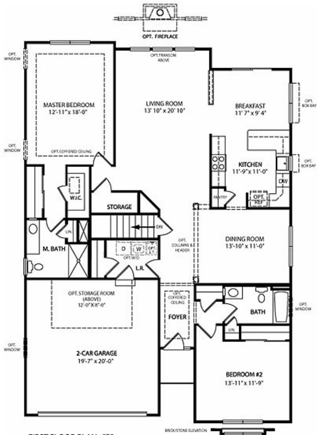
FIRST FLOOR PLAN "B"
