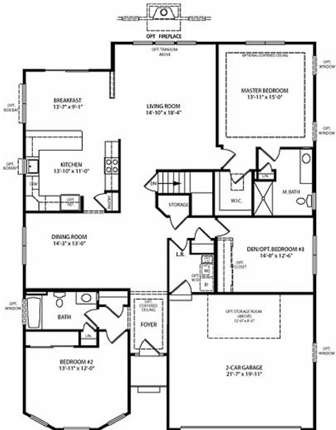
FIRST FLOOR PLAN "D"
